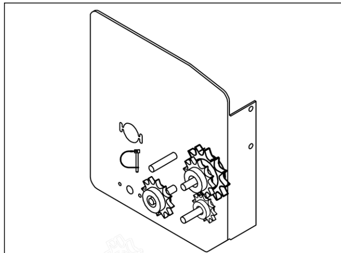
Figure 16 Sprocket Storage
