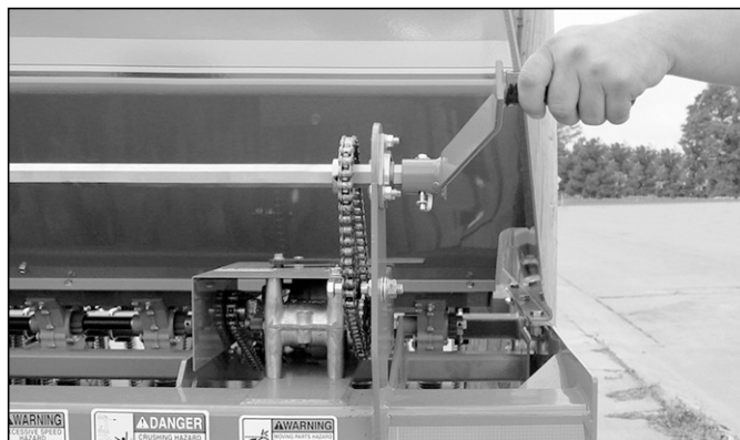
Figure 13 3P606NT Calibration Crank
